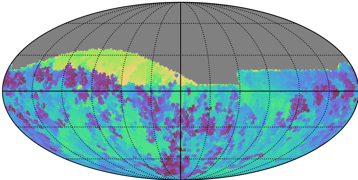
weather_cloudso8v3.4_10yrs Yr 1 all bands: Min skyBrightness
