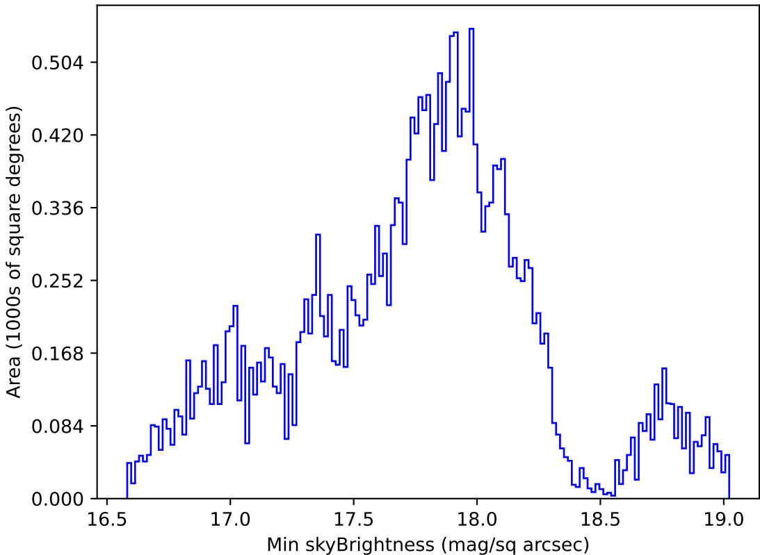
weather_cloudso8v3.4_10yrs Yr 1 all bands: Min skyBrightness
