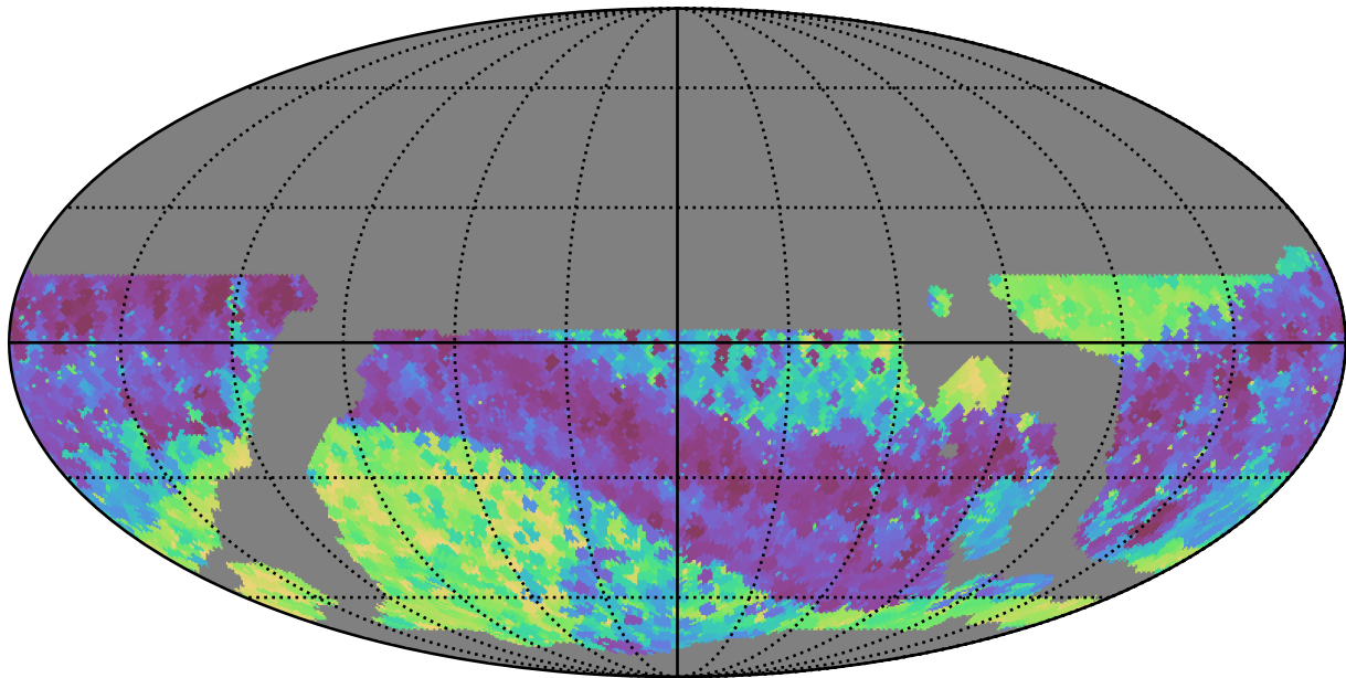
weather_cloudso8v3.4_10yrs WFD z band: Min skyBrightness
