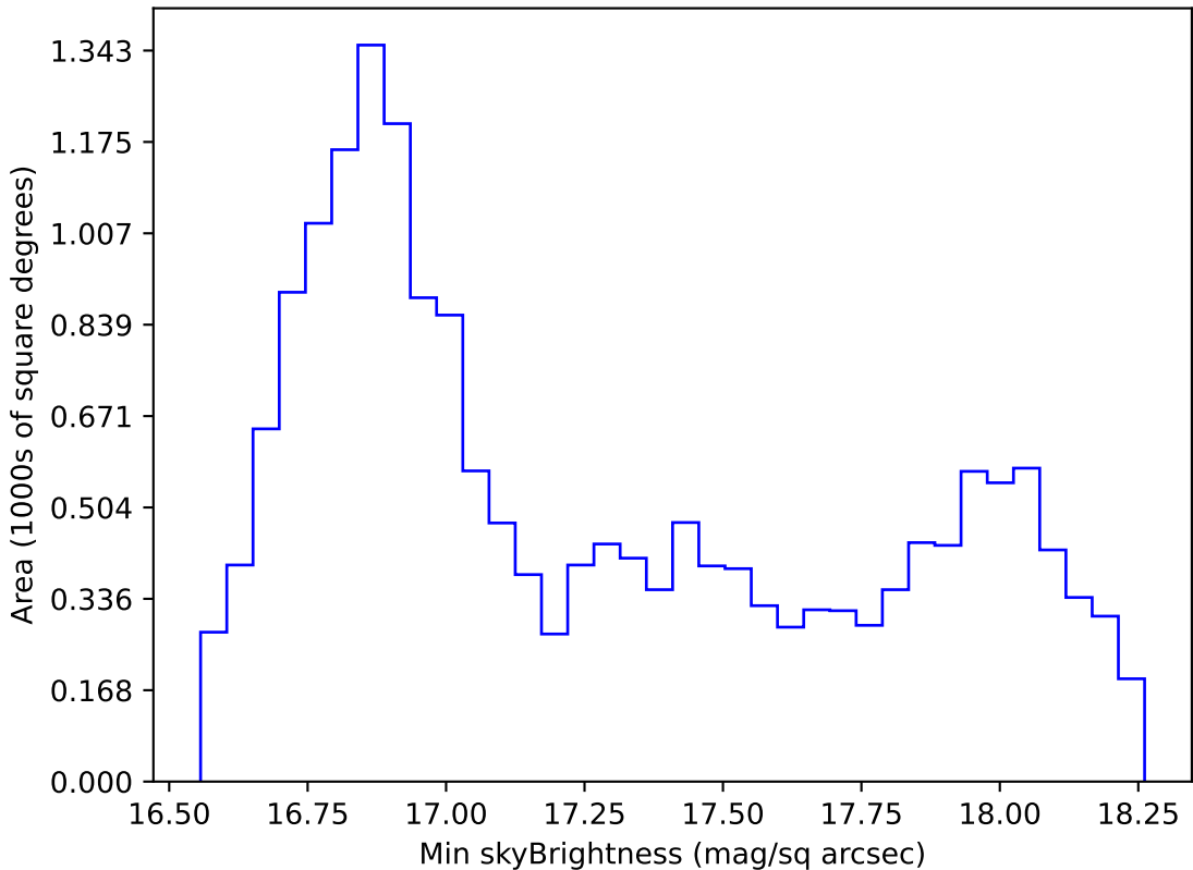
weather_cloudso8v3.4_10yrs WFD z band: Min skyBrightness
