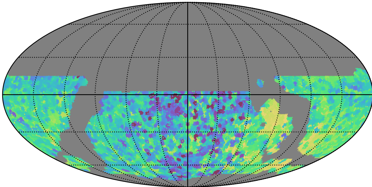
weather_cloudso8v3.4_10yrs WFD y band: Min skyBrightness
