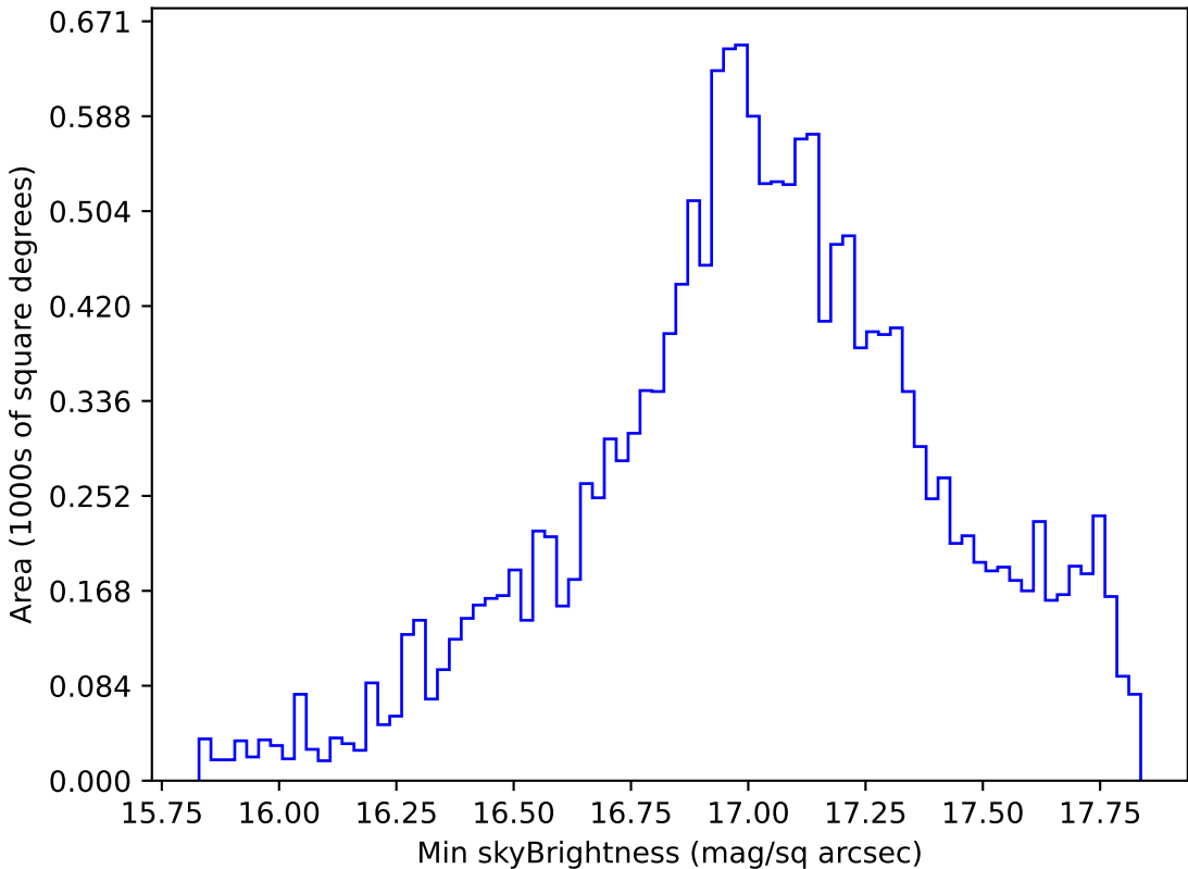
weather_cloudso8v3.4_10yrs WFD y band: Min skyBrightness
