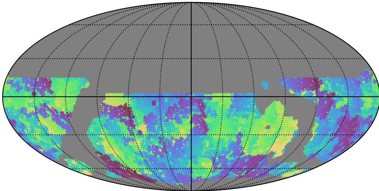
weather_cloudso8v3.4_10yrs WFD u band: Min skyBrightness
