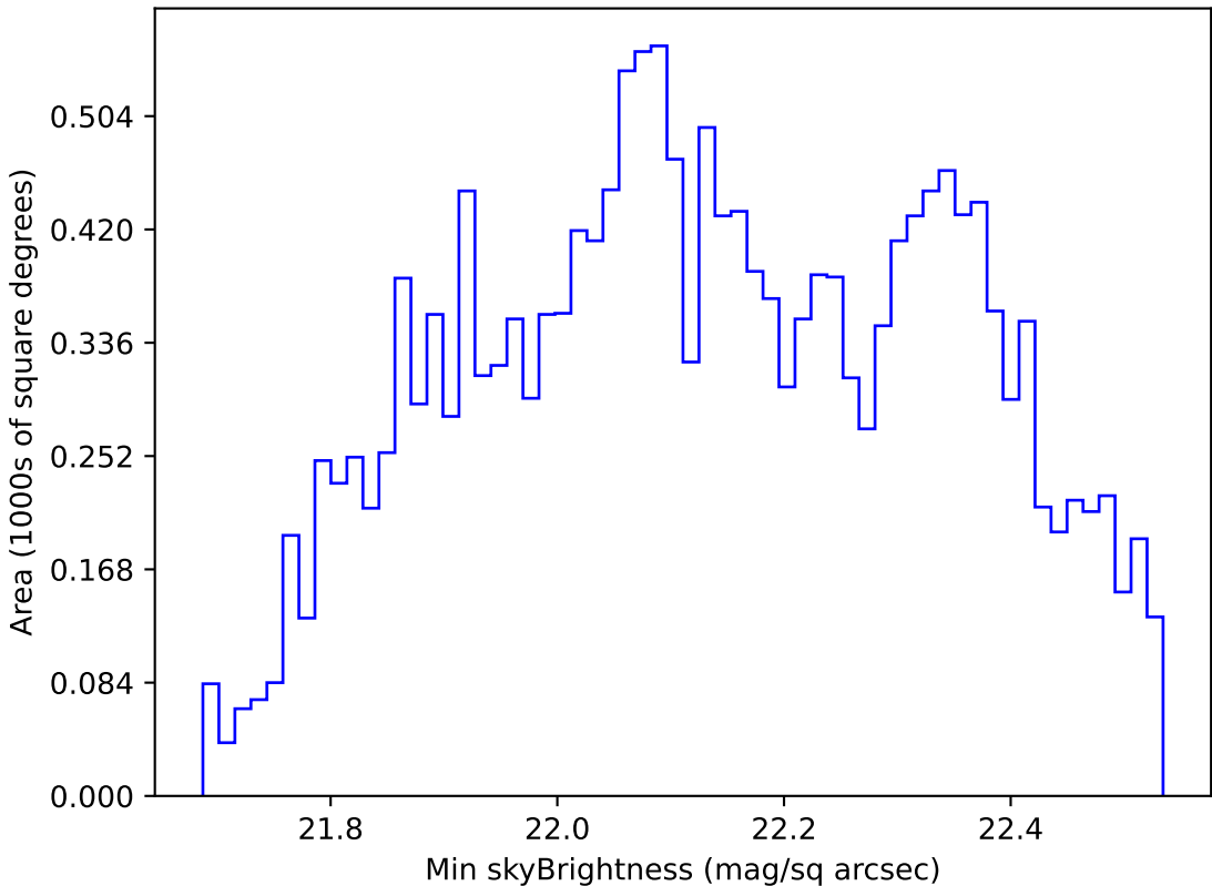
weather_cloudso8v3.4_10yrs WFD u band: Min skyBrightness
