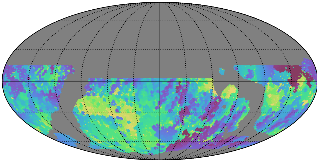
weather_cloudso8v3.4_10yrs WFD r band: Min skyBrightness
