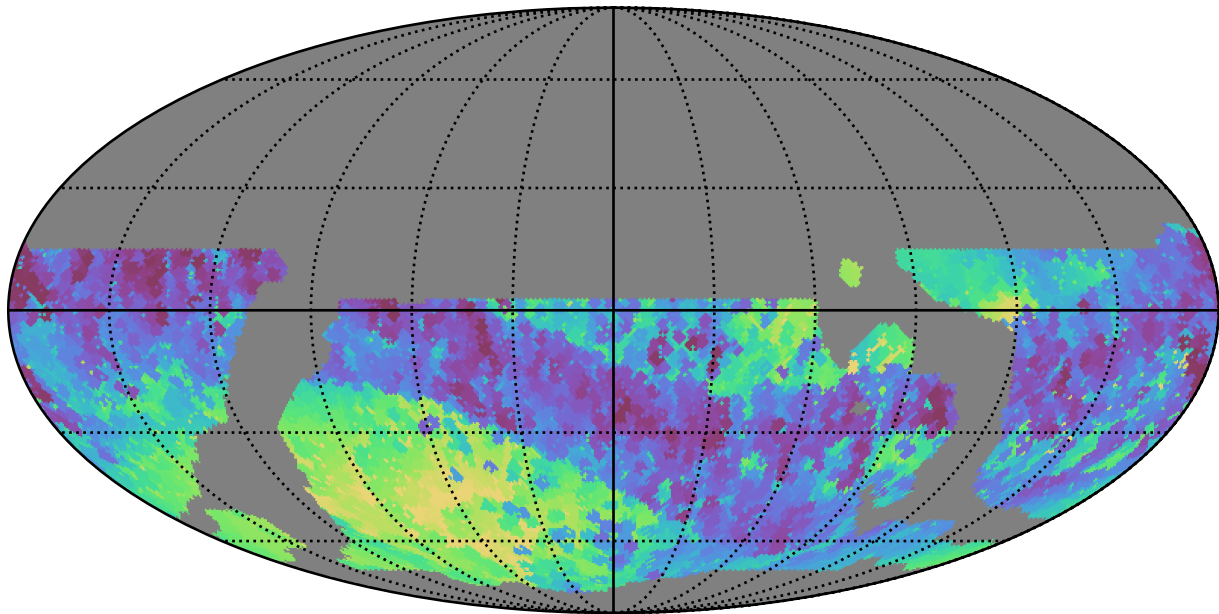
weather_cloudso8v3.4_10yrs WFD i band: Min skyBrightness
