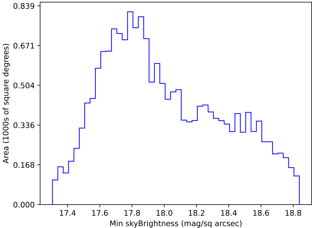
weather_cloudso8v3.4_10yrs WFD i band: Min skyBrightness
