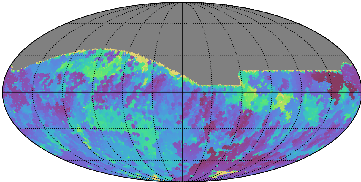
weather_cloudso8v3.4_10yrs All sky r band: Min skyBrightness
