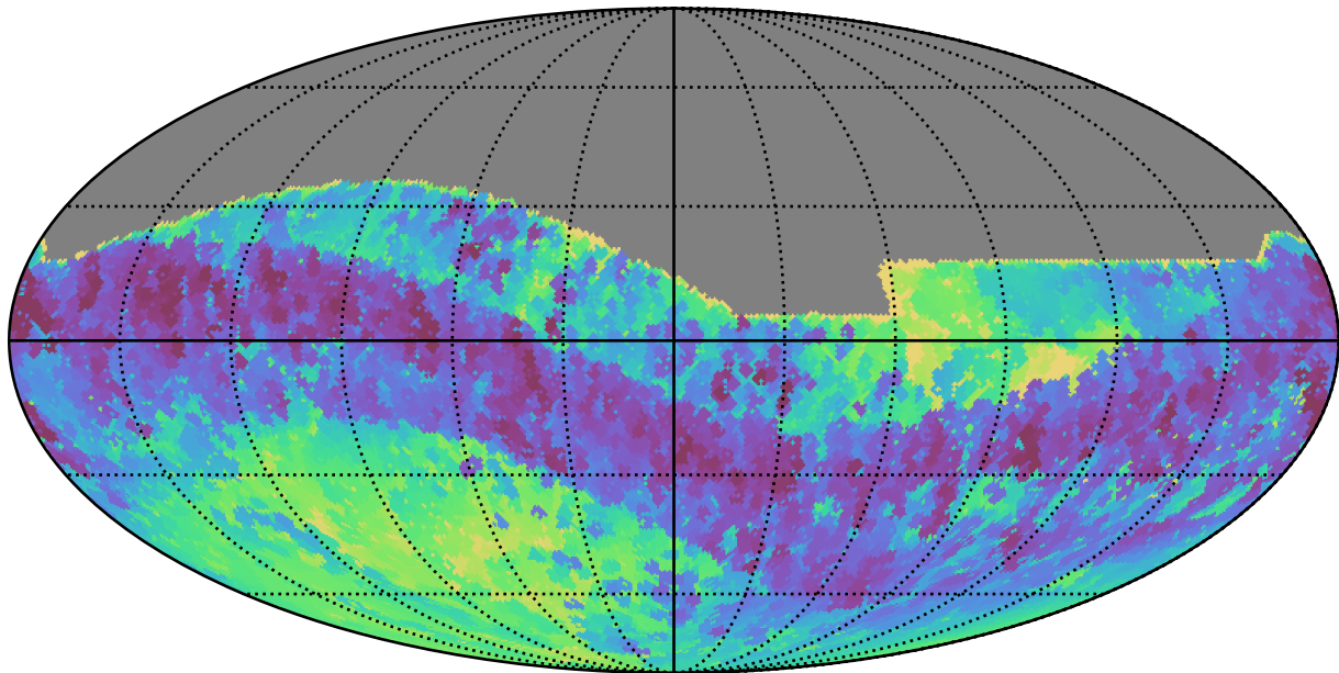
weather_cloudso8v3.4_10yrs All sky i band: Min skyBrightness
