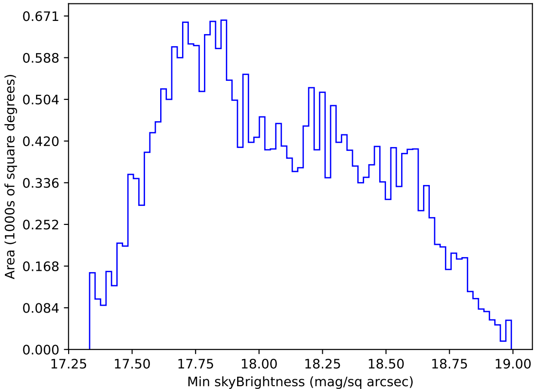
weather_cloudso8v3.4_10yrs All sky i band: Min skyBrightness
