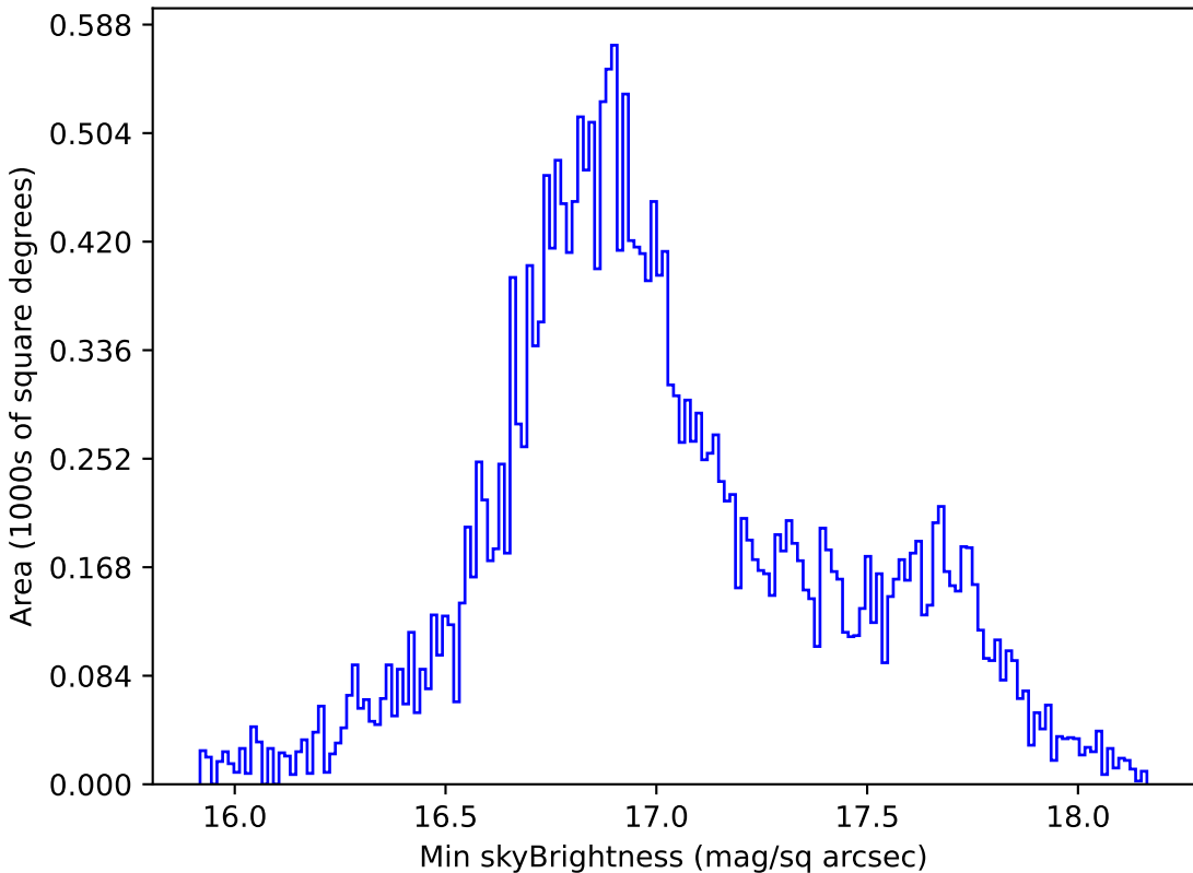
weather_cloudso8v3.4_10yrs All sky all bands: Min skyBrightness
