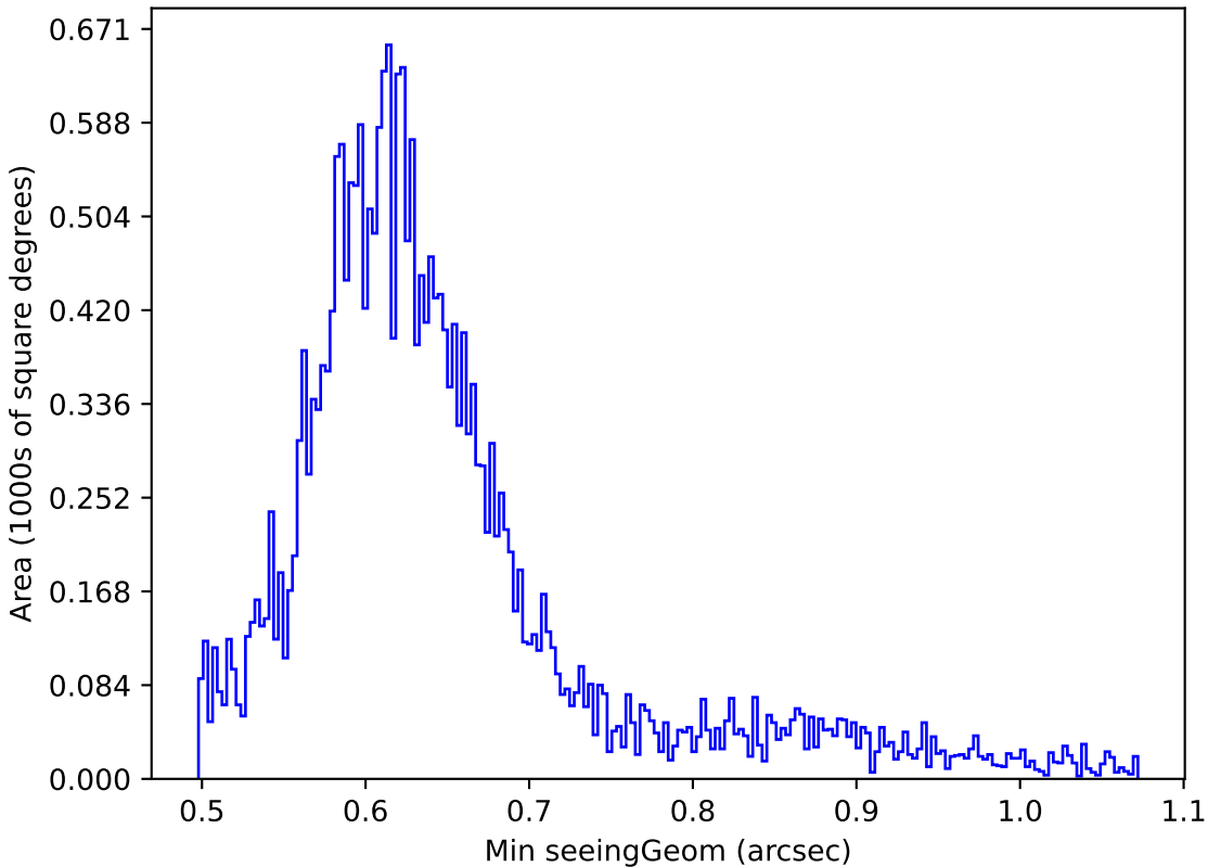
weather_cloudso8v3.4_10yrs Yr 1 r band: Min seeingGeom
