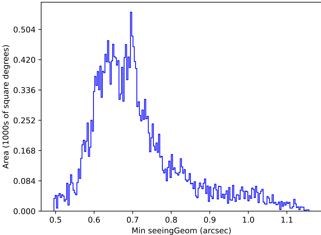
weather_cloudso8v3.4_10yrs Yr 1 g band: Min seeingGeom
