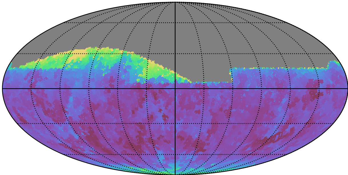
weather_cloudso8v3.4_10yrs Yr 1 all bands: Min seeingGeom
