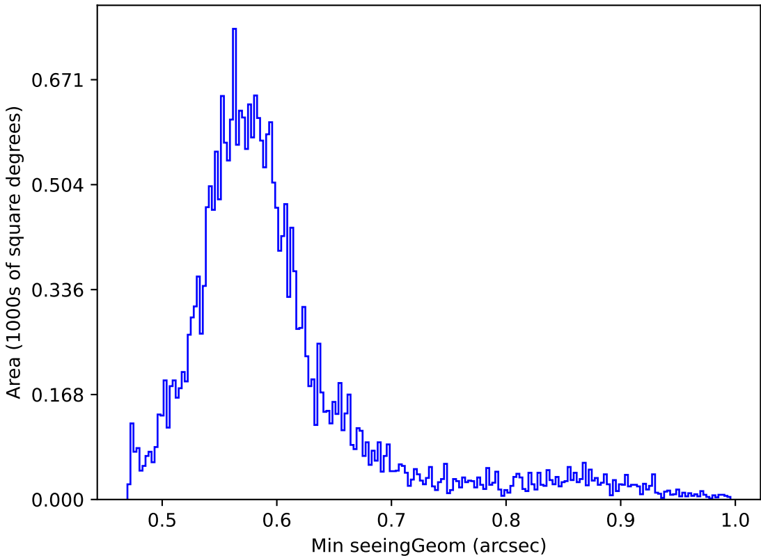
weather_cloudso8v3.4_10yrs Yr 1 all bands: Min seeingGeom
