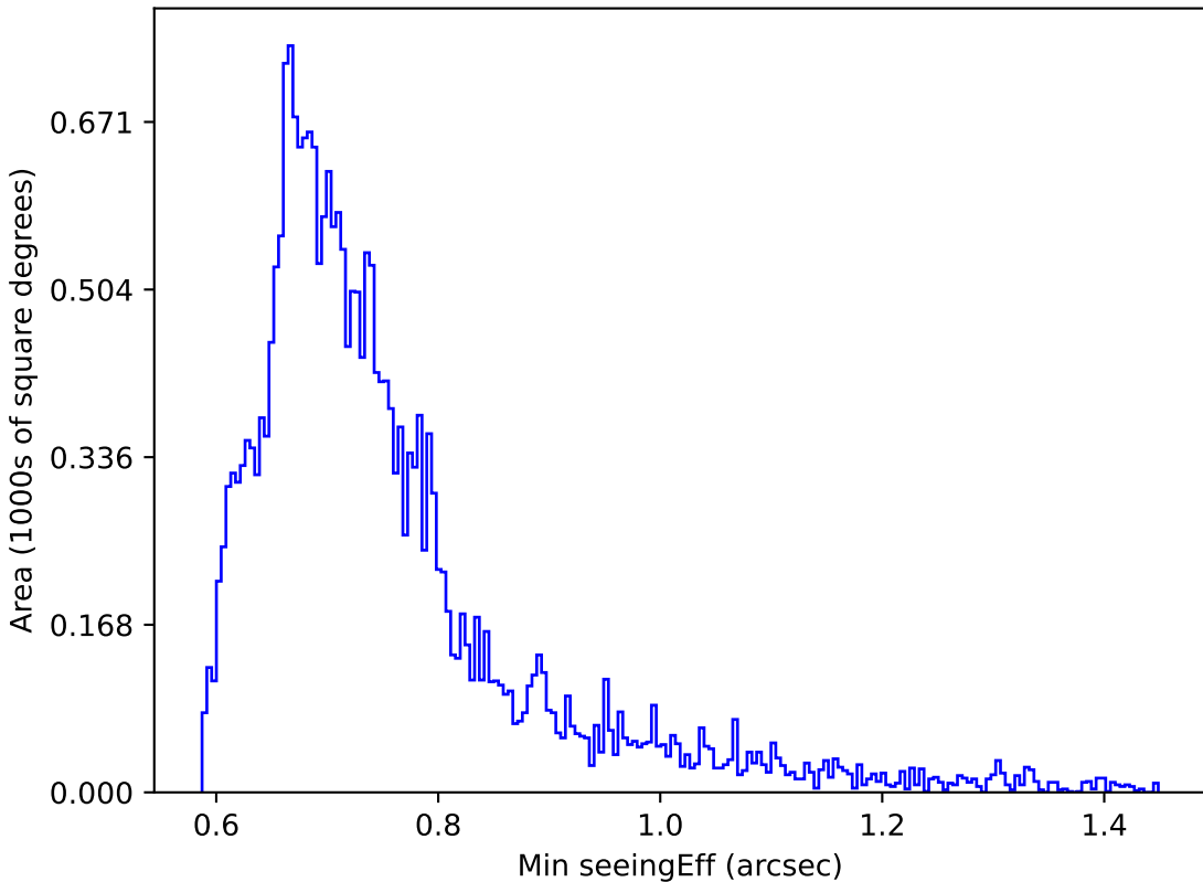
weather_cloudso8v3.4_10yrs Yr 1 z band: Min seeingEff
