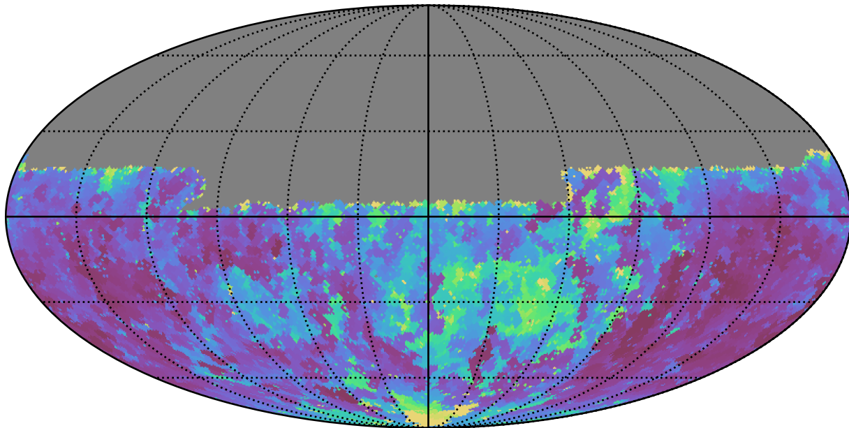
weather_cloudso8v3.4_10yrs Yr 1 u band: Min seeingEff
