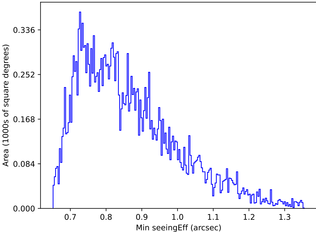
weather_cloudso8v3.4_10yrs Yr 1 u band: Min seeingEff
