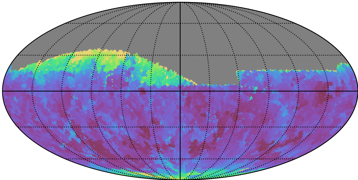
weather_cloudso8v3.4_10yrs Yr 1 r band: Min seeingEff
