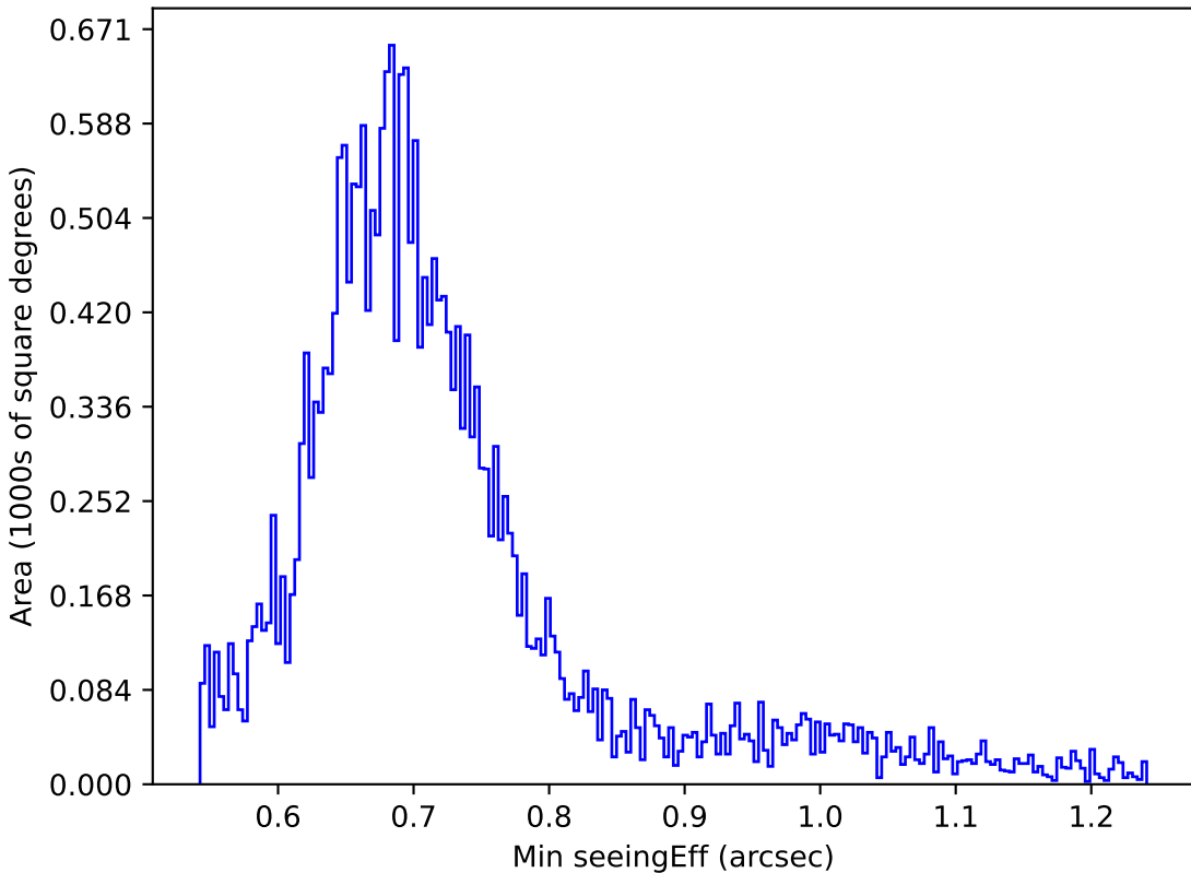
weather_cloudso8v3.4_10yrs Yr 1 r band: Min seeingEff
