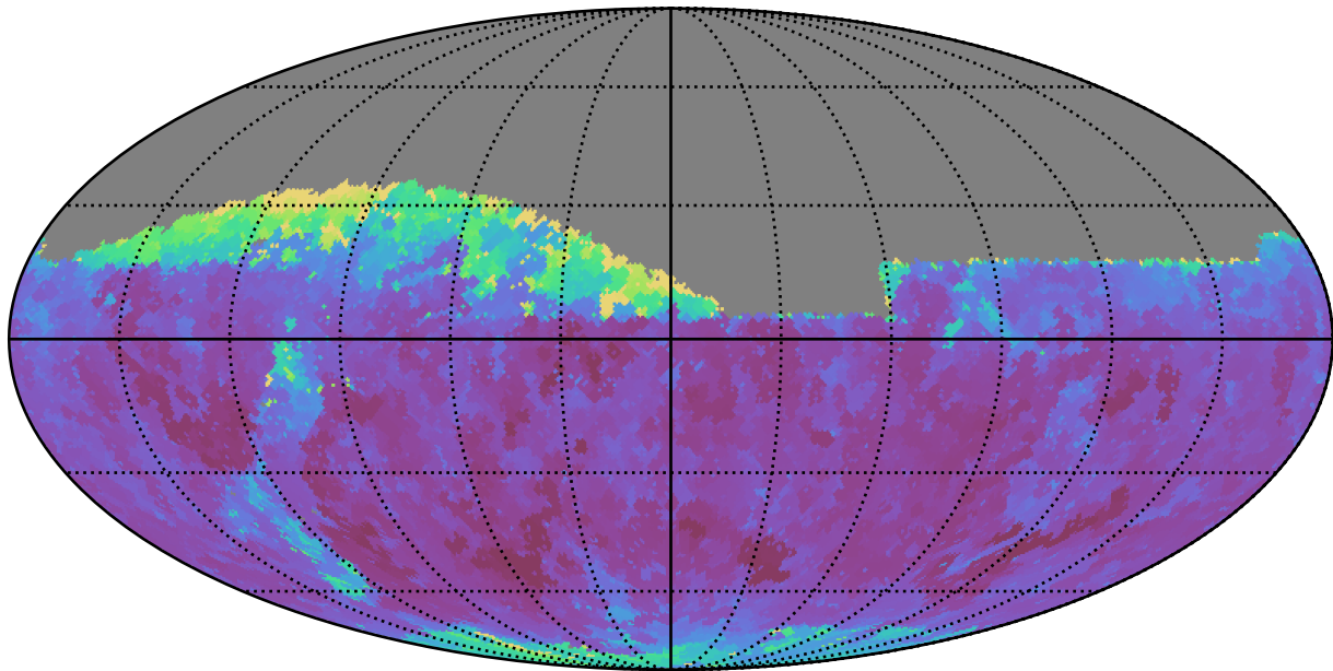
weather_cloudso8v3.4_10yrs Yr 1 i band: Min seeingEff
