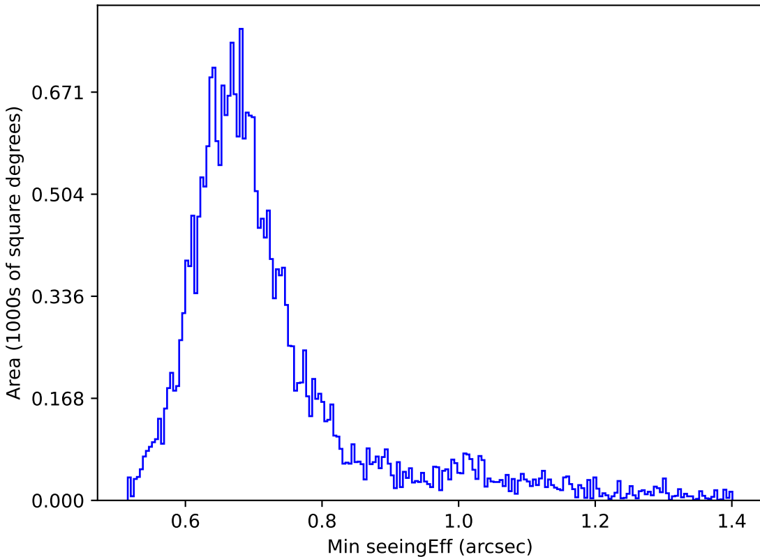
weather_cloudso8v3.4_10yrs Yr 1 i band: Min seeingEff
