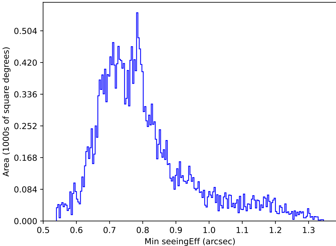
weather_cloudso8v3.4_10yrs Yr 1 g band: Min seeingEff
