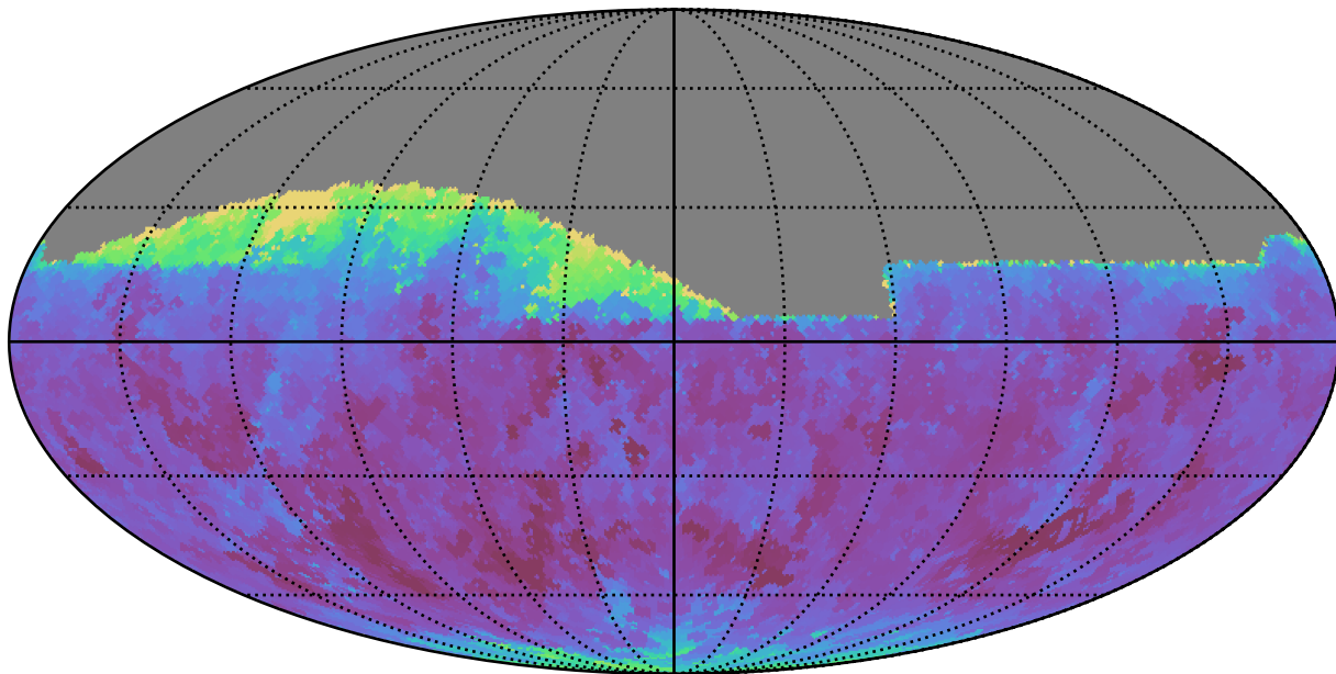
weather_cloudso8v3.4_10yrs Yr 1 all bands: Min seeingEff
