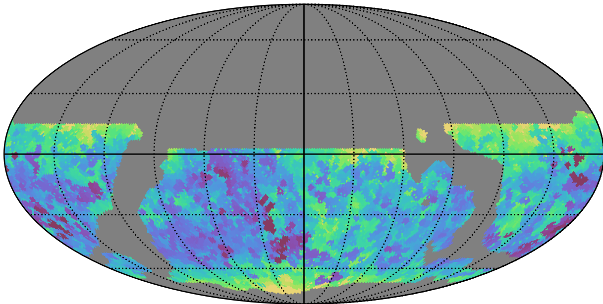
weather_cloudso8v3.4_10yrs WFD z band: Min seeingEff
