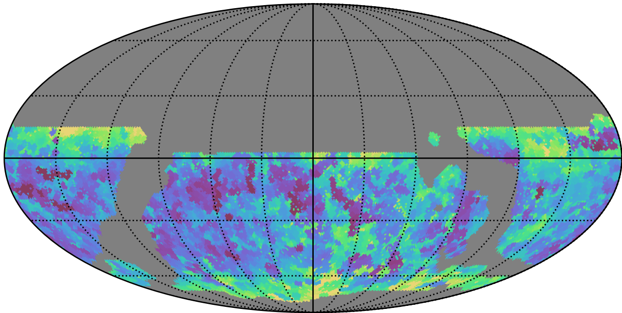
weather_cloudso8v3.4_10yrs WFD y band: Min seeingEff
