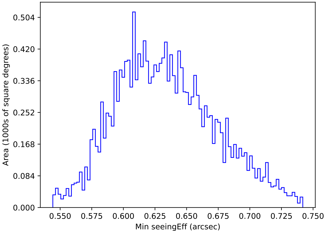
weather_cloudso8v3.4_10yrs WFD y band: Min seeingEff
