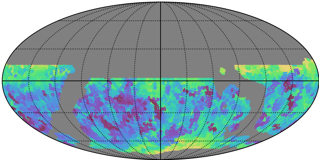
weather_cloudso8v3.4_10yrs WFD r band: Min seeingEff
