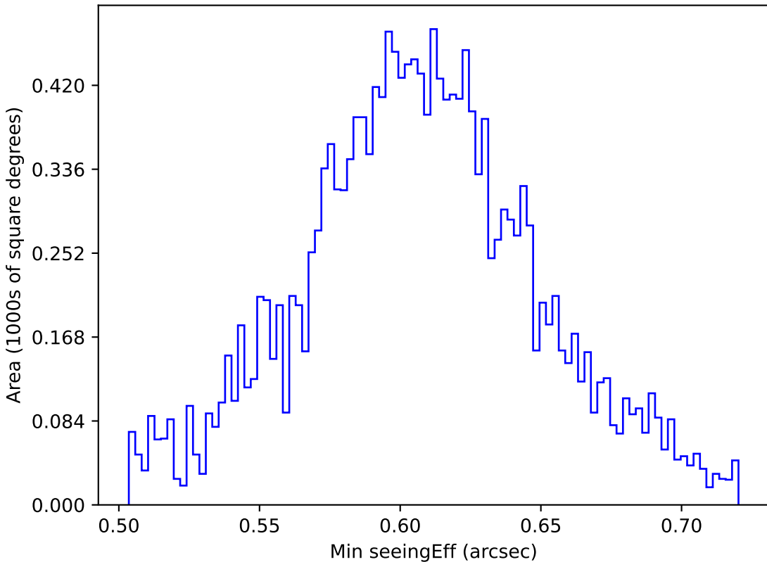
weather_cloudso8v3.4_10yrs WFD i band: Min seeingEff
