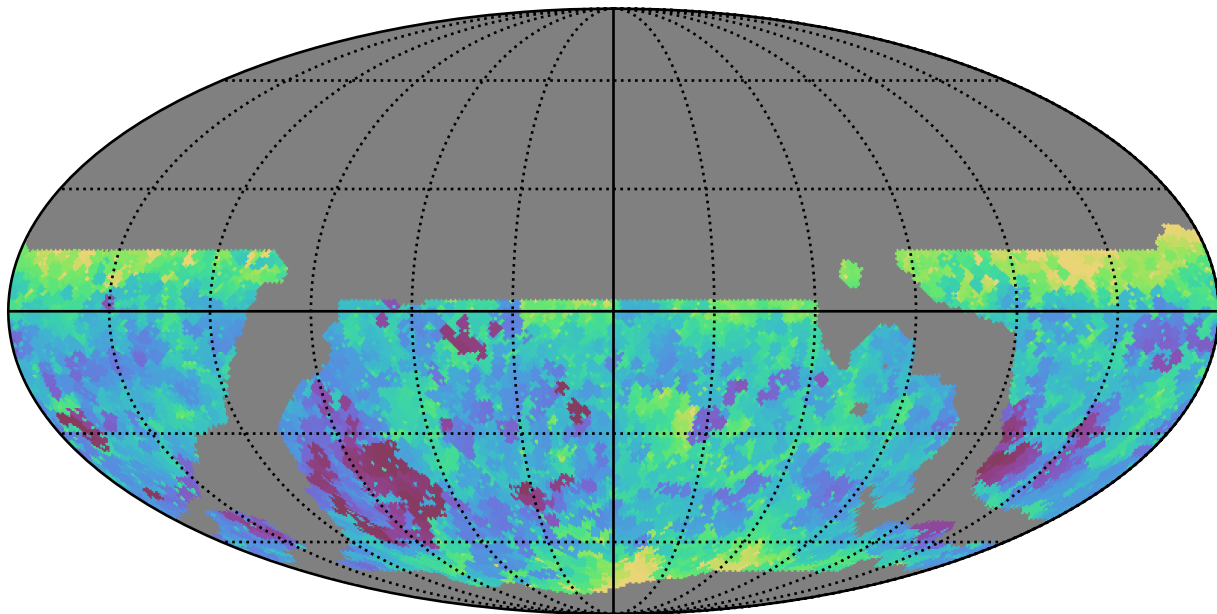
weather_cloudso8v3.4_10yrs WFD g band: Min seeingEff
