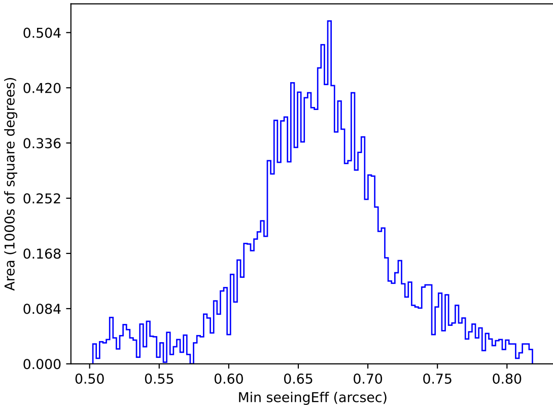
weather_cloudso8v3.4_10yrs WFD g band: Min seeingEff
