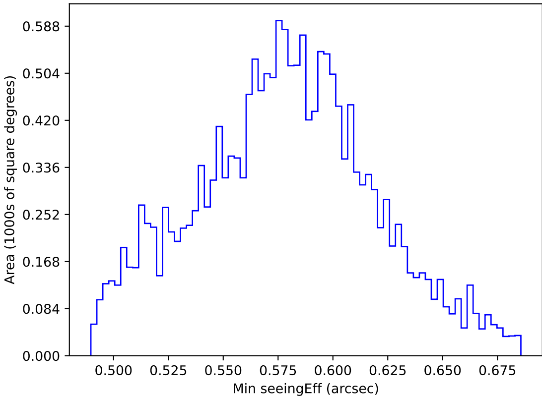
weather_cloudso8v3.4_10yrs WFD all bands: Min seeingEff
