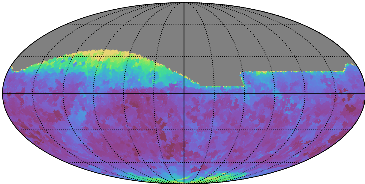
weather_cloudso8v3.4_10yrs All sky z band: Min seeingEff
