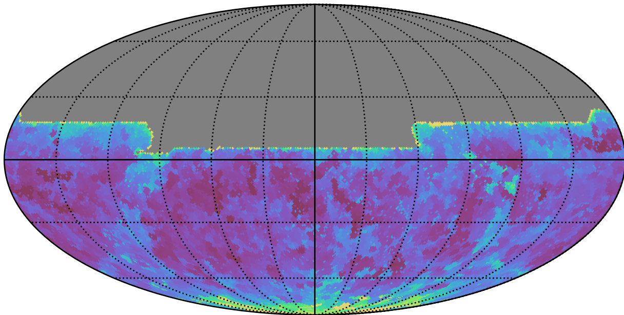
weather_cloudso8v3.4_10yrs All sky y band: Min seeingEff
