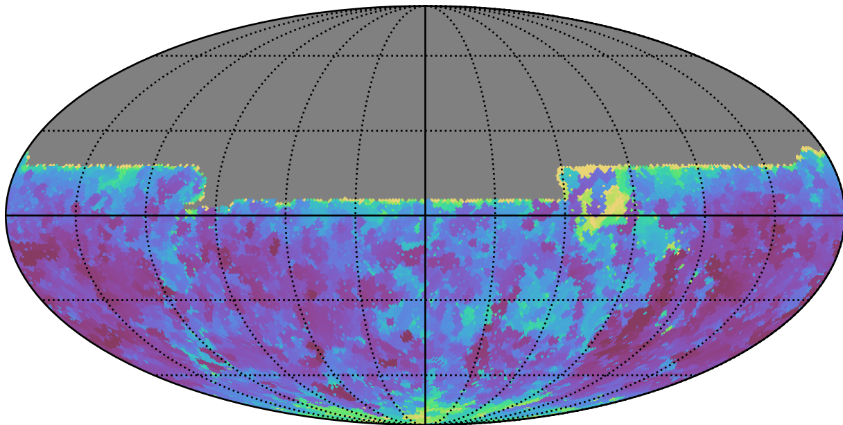
weather_cloudso8v3.4_10yrs All sky u band: Min seeingEff
