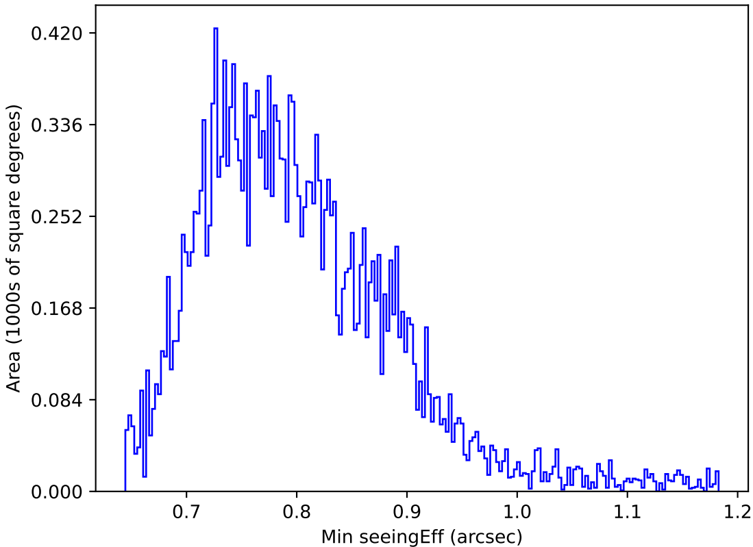
weather_cloudso8v3.4_10yrs All sky u band: Min seeingEff
