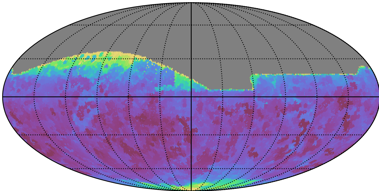
weather_cloudso8v3.4_10yrs All sky r band: Min seeingEff
