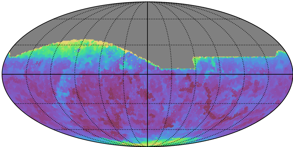
weather_cloudso8v3.4_10yrs All sky i band: Min seeingEff
