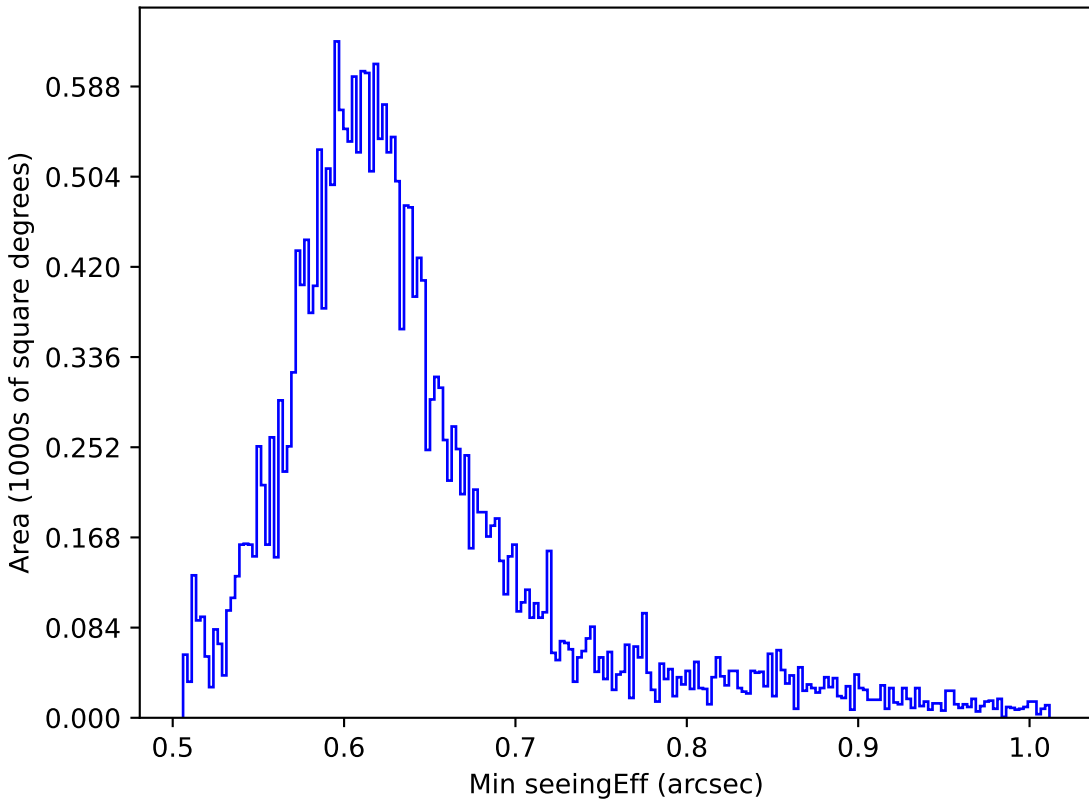
weather_cloudso8v3.4_10yrs All sky i band: Min seeingEff
