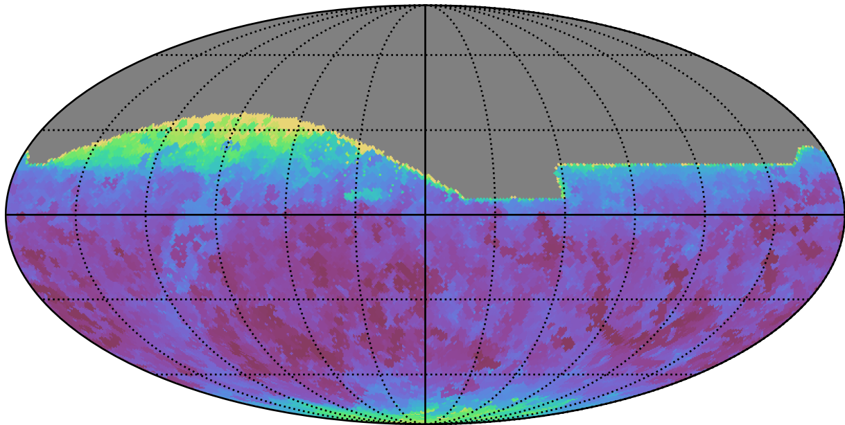
weather_cloudso8v3.4_10yrs All sky all bands: Min seeingEff
