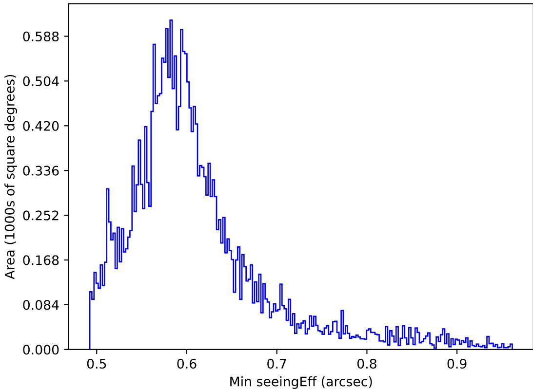
weather_cloudso8v3.4_10yrs All sky all bands: Min seeingEff
