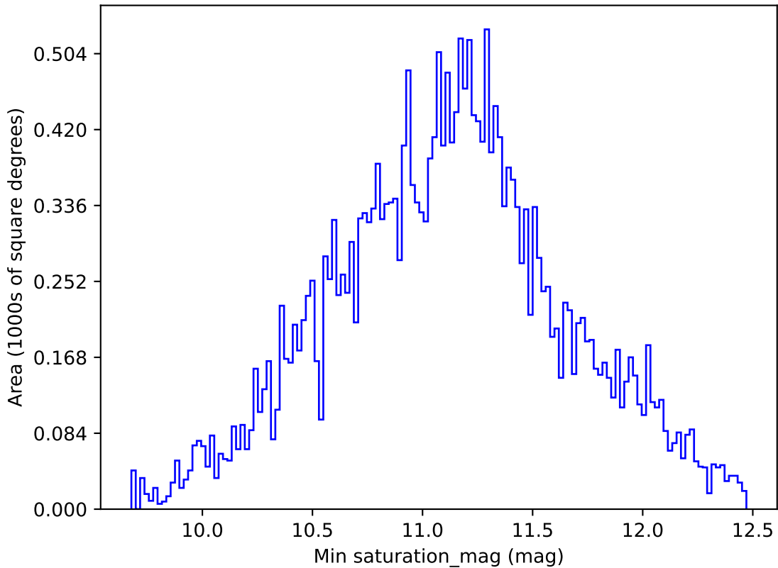
weather_cloudso8v3.4_10yrs All sky all bands: Min saturation_mag
