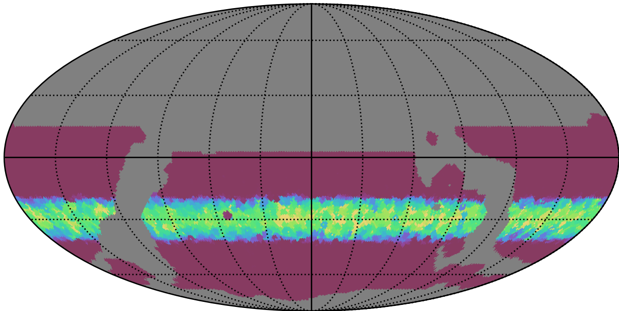
weather_cloudso8v3.4_10yrs WFD z band: Min normairmass
