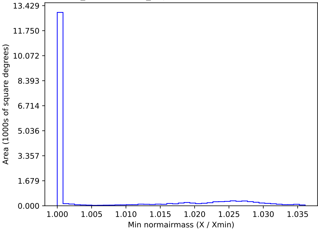
weather_cloudso8v3.4_10yrs WFD z band: Min normairmass
