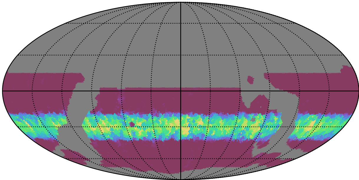
weather_cloudso8v3.4_10yrs WFD u band: Min normairmass
