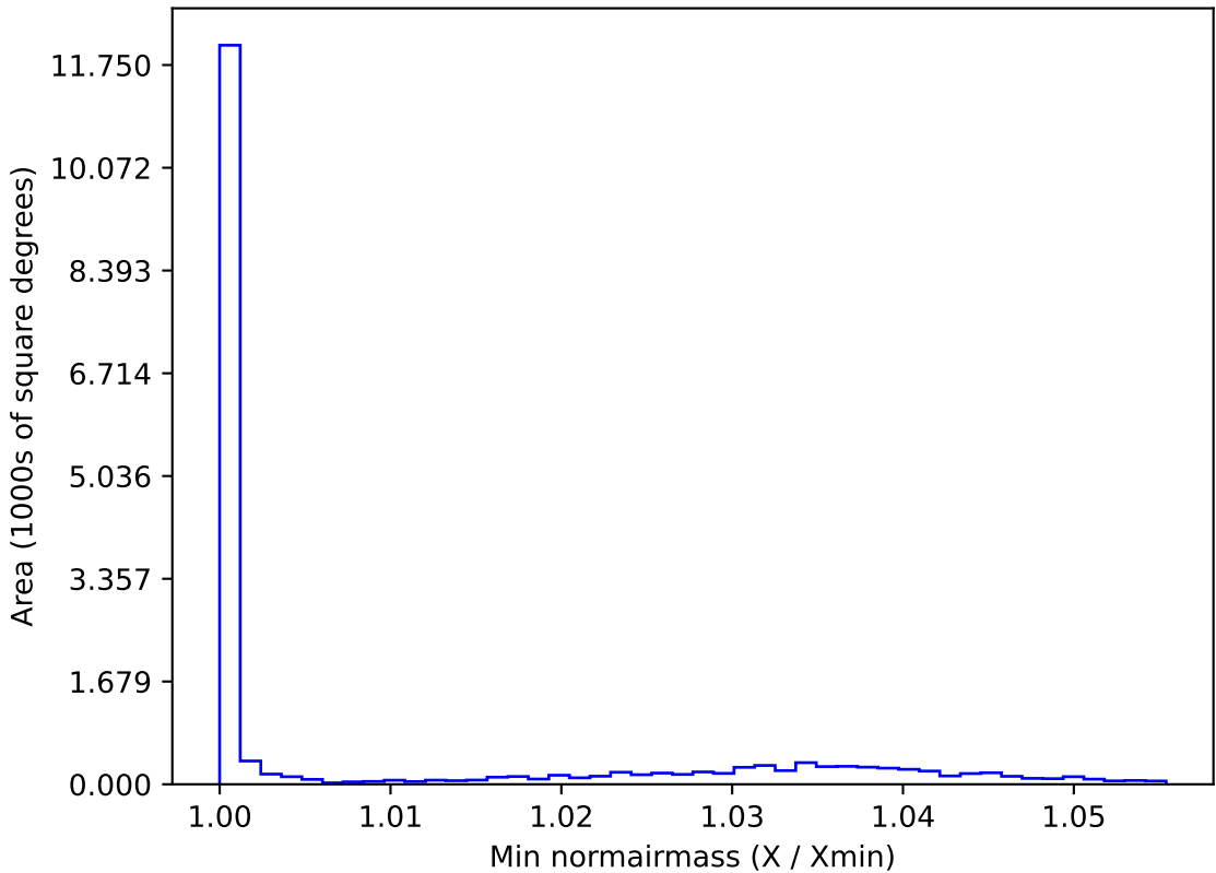
weather_cloudso8v3.4_10yrs WFD u band: Min normairmass
